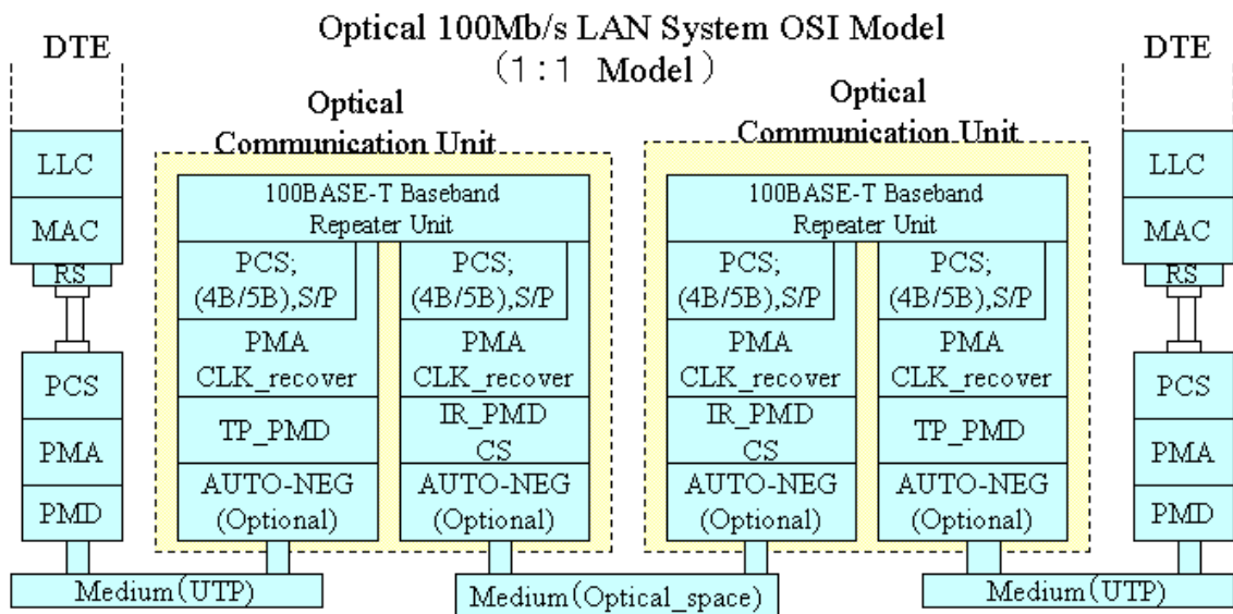
Fig. 7-1 Typical topology of a one-to-one system
