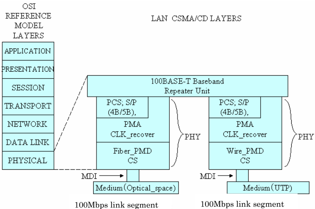
Fig. 5-2 OSI model for an optical wireless device
