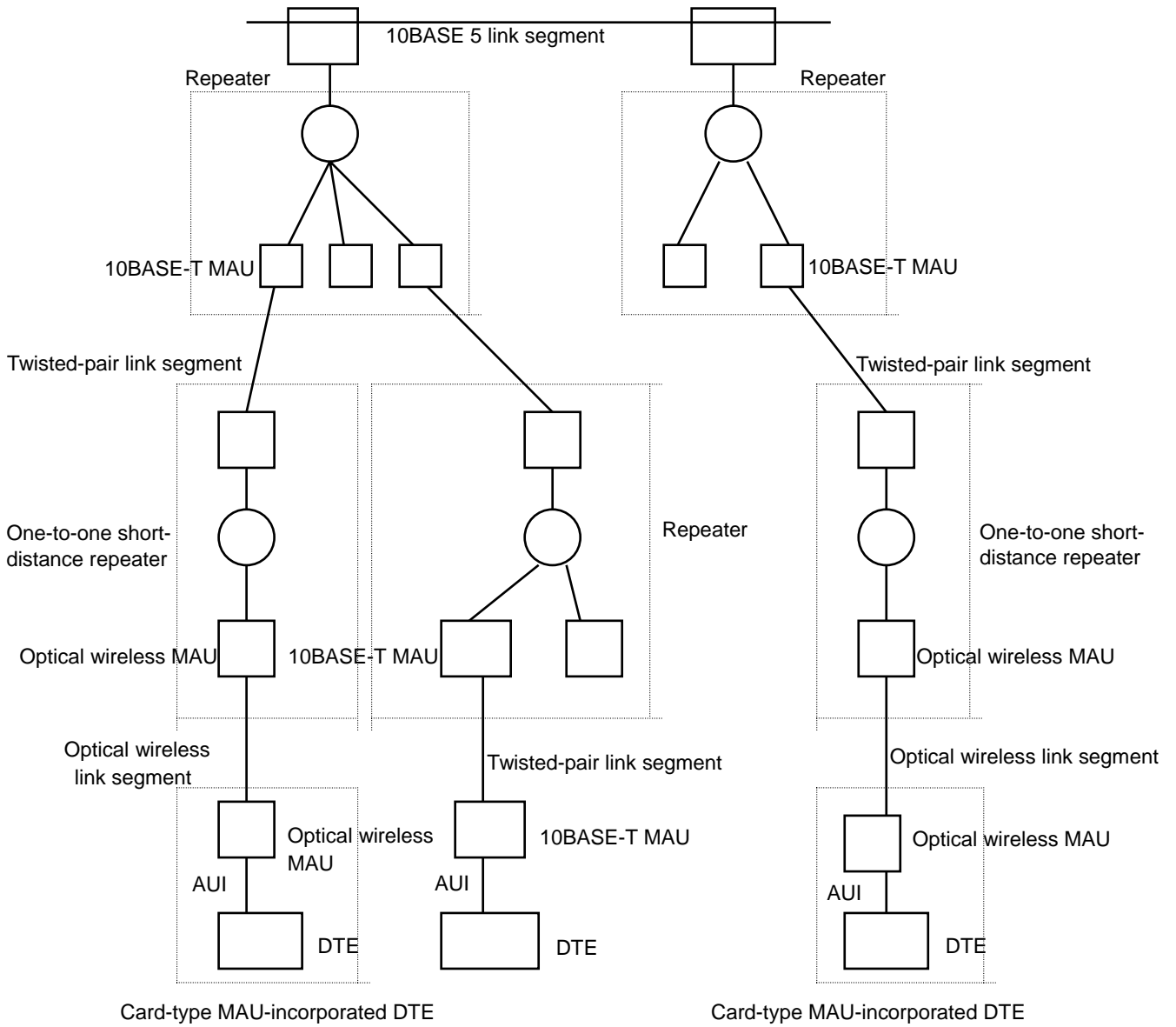
Fig. 4-3 Typical topology of a one-to-one short-distance system
