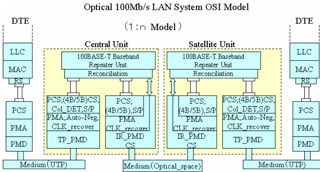
Fig. 7-2 Typical topology of a one-to-n system
