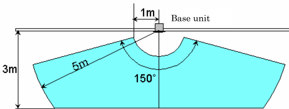
Fig. 8-1 Typical beam profile representation
