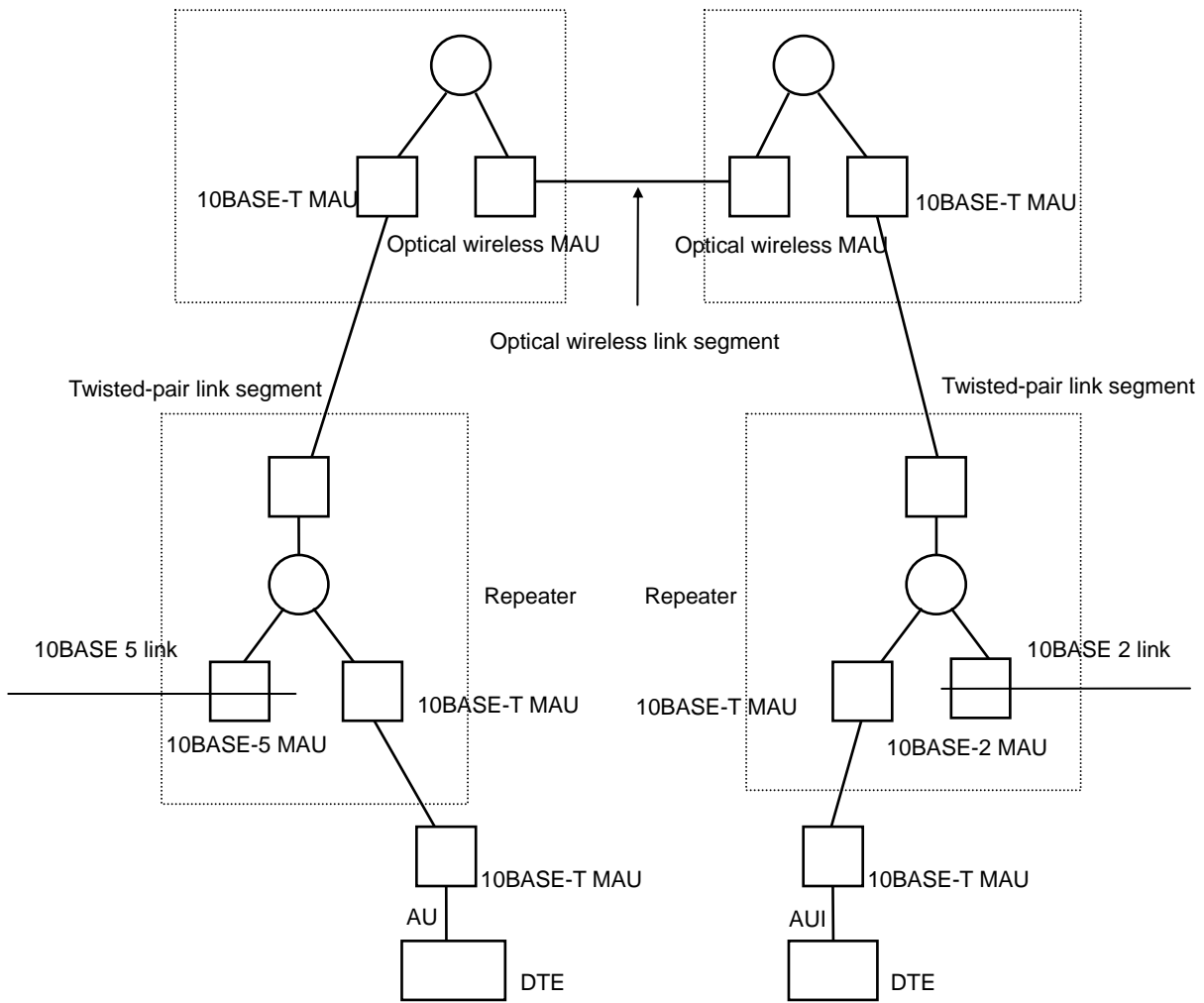
Fig. 4-1 Typical topology of a one-to-one long-distance system
